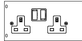
FBIL036/ FBILST036 UK 2G 13A SWITCHED SOCKET -LEFT HANDED (DOUBLE POLE)
